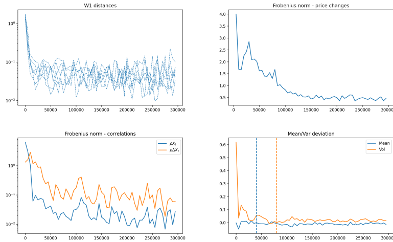
Figure 4: Convergence WGAN-GP with Gradient Clipping.
